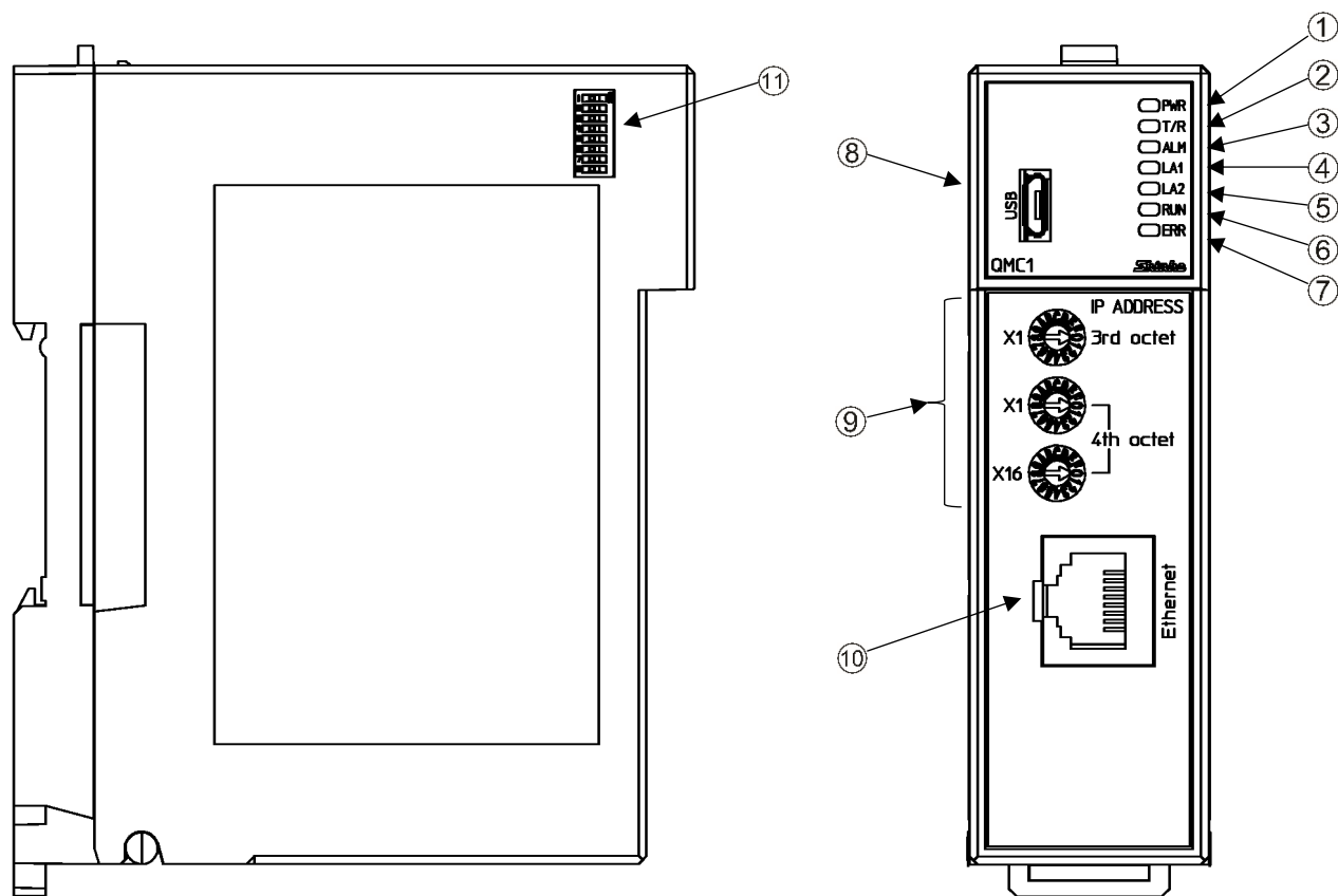
Base part
